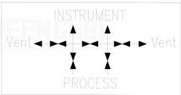
DETAIL OF MANIFOLD
